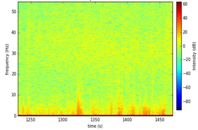
Spectrogram for rb rec171 (S23) zazen, post post
