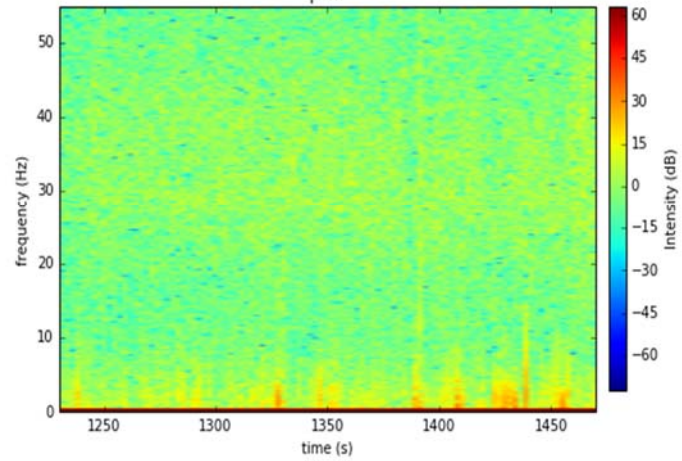
Spectrogram for lb rec171 (S23) zazen, post post
