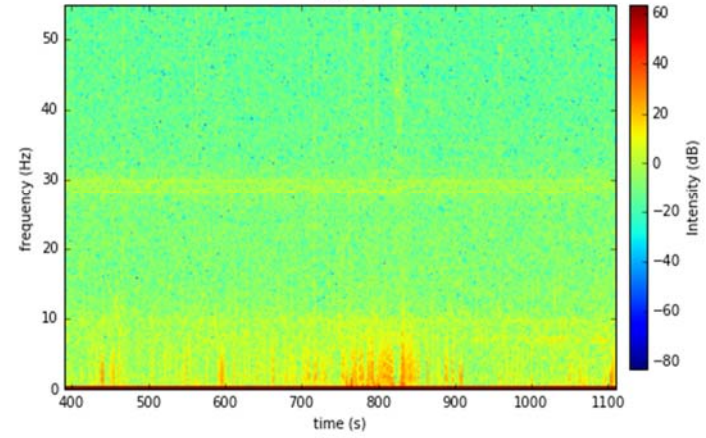
Spectrogram for rb rec183 (S31) pre, zazen, post zazen
