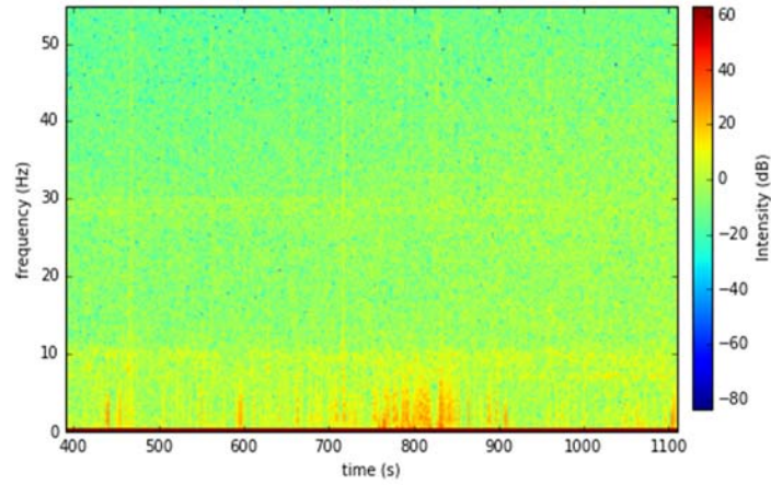
Spectrogram for lb rec183 (S31) pre, zazen, post zazen
