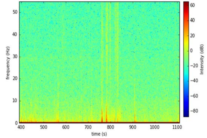
Spectrogram for rb rec183 (S31) pre, zazen, post zazen
