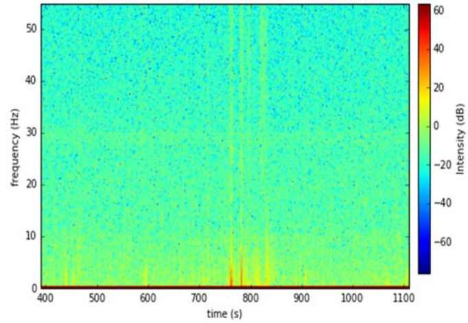
Spectrogram for lb rec183 (S31) pre, zazen, post zazen
