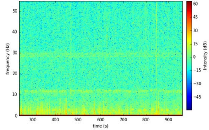
Spectrogram for rb rec172 (S24) zazen, post zazen
