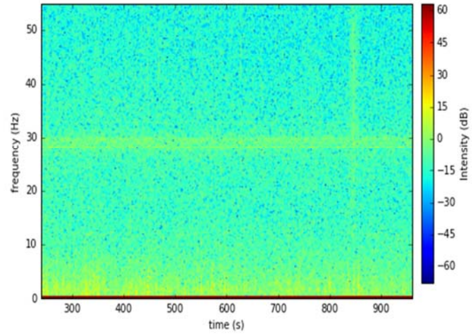
Spectrogram for lb rec172 (S24) zazen, post zazen
