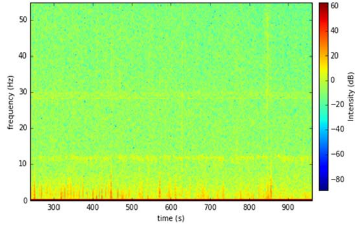
Spectrogram for lb rec172 (S24) zazen, post zazen
