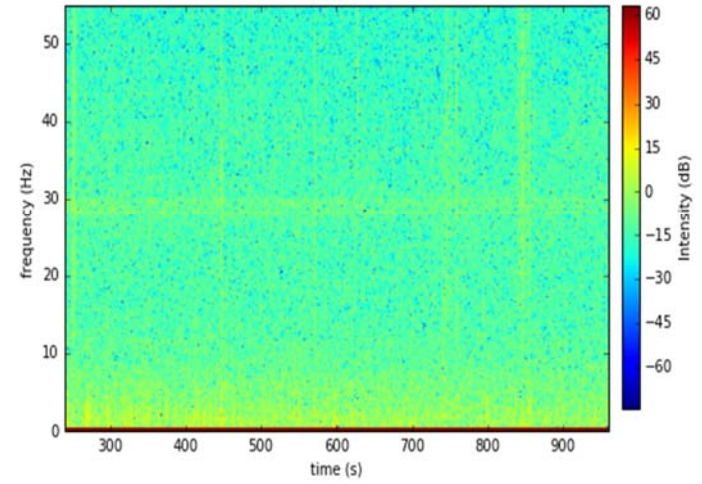
Spectrogram for rb rec172 (S24) zazen, post zazen
