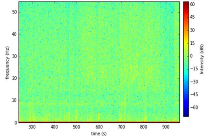
Spectrogram for rb rec173 (S1) zazen, post zazen
