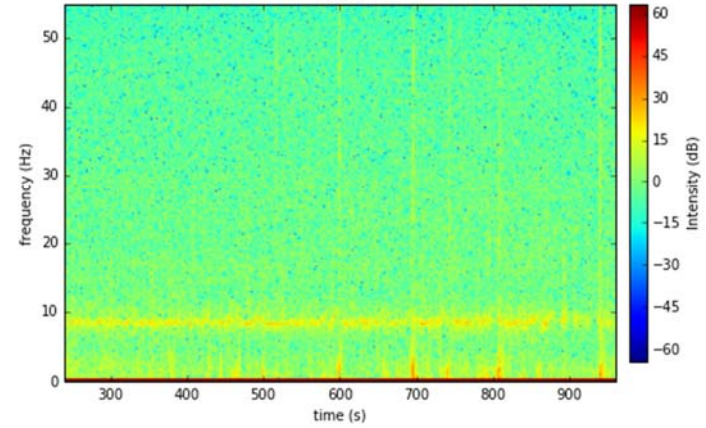
Spectrogram for rb rec173 (S1) zazen, post zazen
