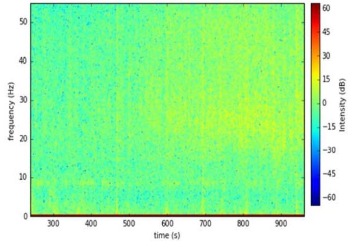
Spectrogram for lb rec173 (S1) zazen, post zazen
