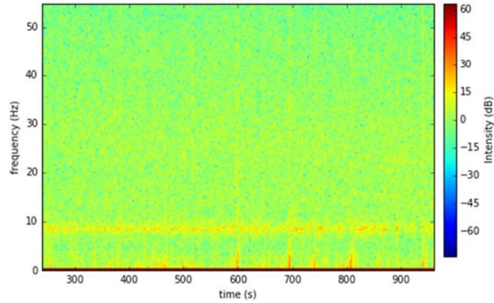
Spectrogram for lb rec173 (S1) zazen, post zazen
